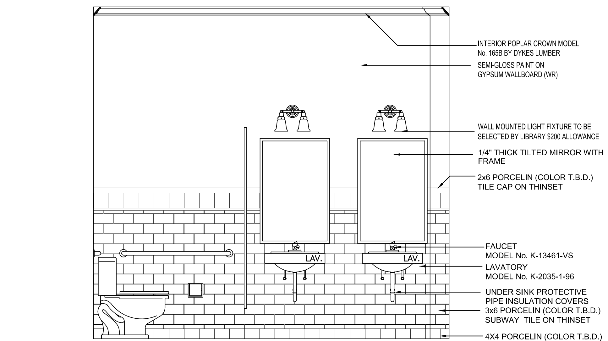
2 TYPICAL MULTI-STALL ADA COMPLIANT BATHROOM INTERIOR ELEVATIONS SCALE: 1/2" = 1'-0"
