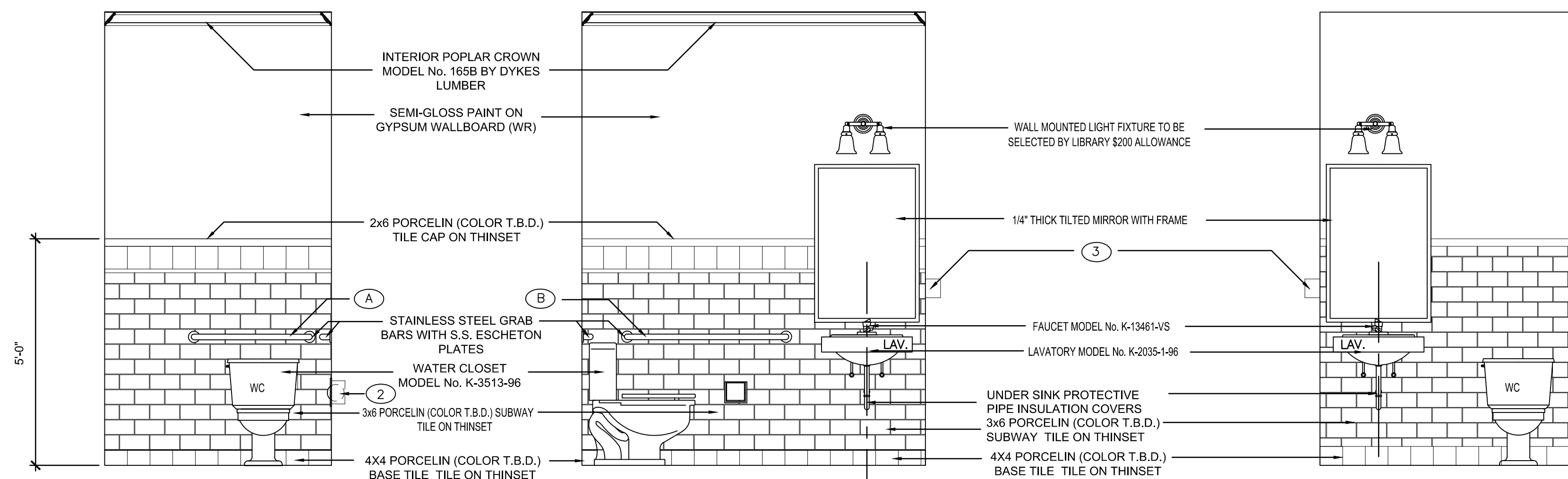
1 TYPICAL SINGLE ADA COMPLIANT BATHROOM INTERIOR ELEVATIONS SCALE: 1/2" = 1'-0"
