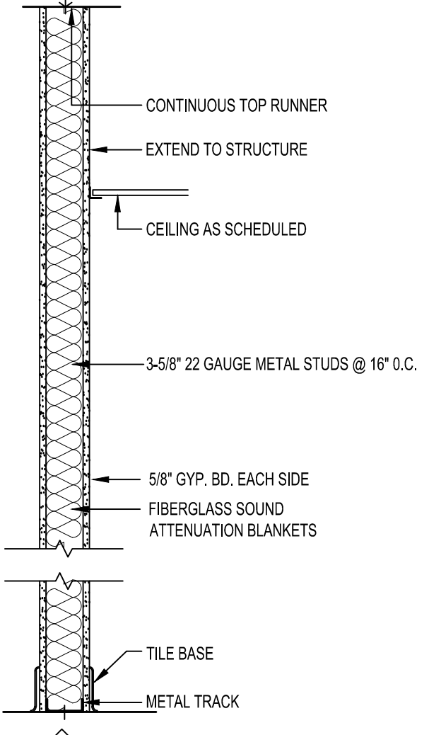
1 TYPICAL NEW WALL TO MATCH BUILDING STANDARD, VERIFY IN FIELD
